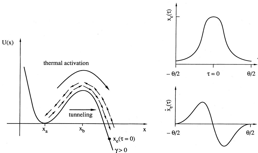
FIG. 38. Potential U(x) used in the description of the quantum-Kramers rate. The periodic bounce trajectory x_e(\tau) , with period \hbar\beta = \theta , describes low-temperature tunneling under the barrier and is a stationary point of the Euclidean action in Eq. (9.6), obeying the classical equation of motion in the inverted potential -U(x) [see Eq. (9.12)]. The Goldstone mode \propto \dot{x}_e(\tau) processes one node; i.e., there is a fluctuation mode with a negative eigenvalue. The point marked x_e(\tau=0) gives the zero-temperature bounce point in the presence of finite damping \gamma , which characterizes the loss of energy during tunneling under frictional influence (Weiss et al. , 1984).
